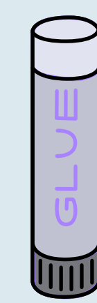
GLUE
